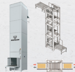
Continuous Lifter
