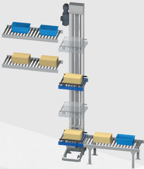
Reciprocating Vertical Conveyor
